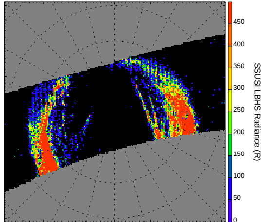
Northern Hemisphere 20 Nov 23:00 UT
