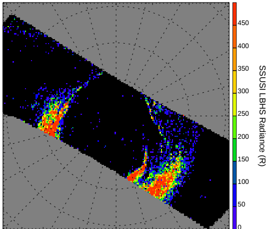
Northern Hemisphere 21 Nov 13:29 UT
