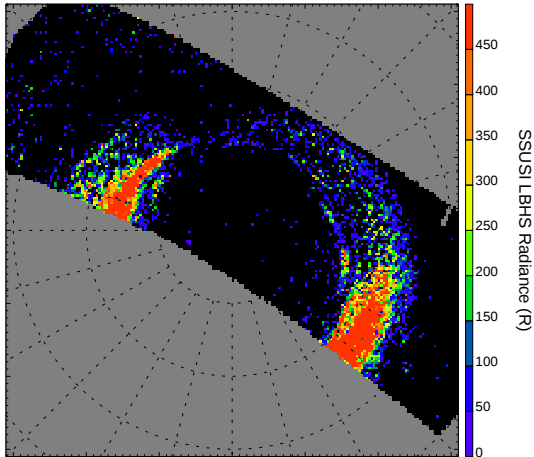
Northern Hemisphere 20 Nov 23:51 UT
