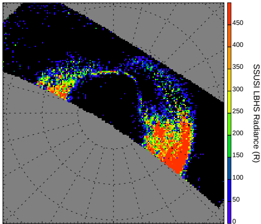
Northern Hemisphere 21 Nov 01:34 UT
