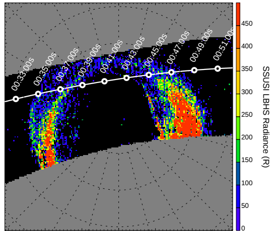
Northern Hemisphere 21 Nov 00:42 UT
