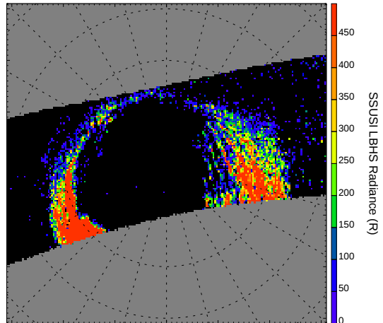
Northern Hemisphere 21 Nov 12:38 UT
