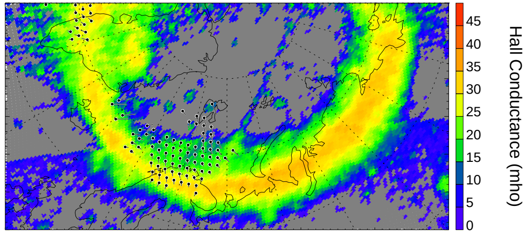
Hall Conductance from IMAGE/WIC
