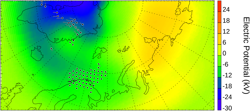
Electric Potential from SuperDARN 20:22:00 - 20:24:00 UT
