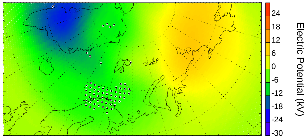
Electric Potential from SuperDARN 20:20:00 - 20:22:00 UT
