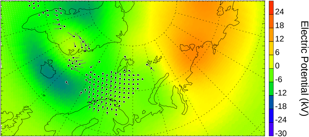
Electric Potential from SuperDARN 20:30:00 - 20:32:00 UT
