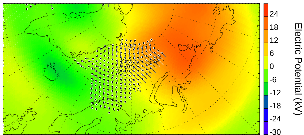
Electric Potential from SuperDARN 20:36:00 - 20:38:00 UT
