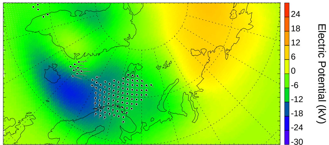
Electric Potential from SuperDARN 20:28:00 - 20:30:00 UT
