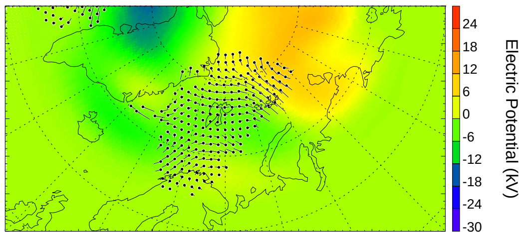
Electric Potential from SuperDARN 20:42:00 - 20:44:00 UT
