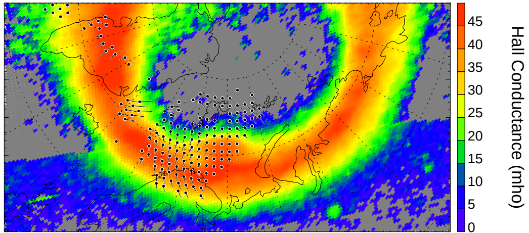
Hall Conductance from IMAGE/WIC
