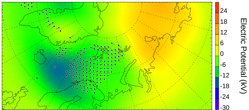
Electric Potential from SuperDARN 20:32:00 - 20:34:00 UT
