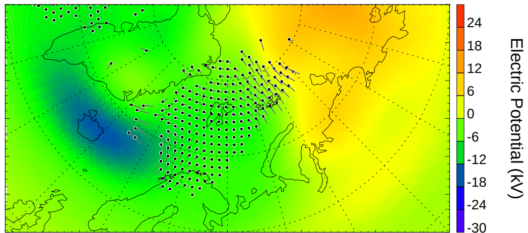
Electric Potential from SuperDARN 20:40:00 - 20:42:00 UT
