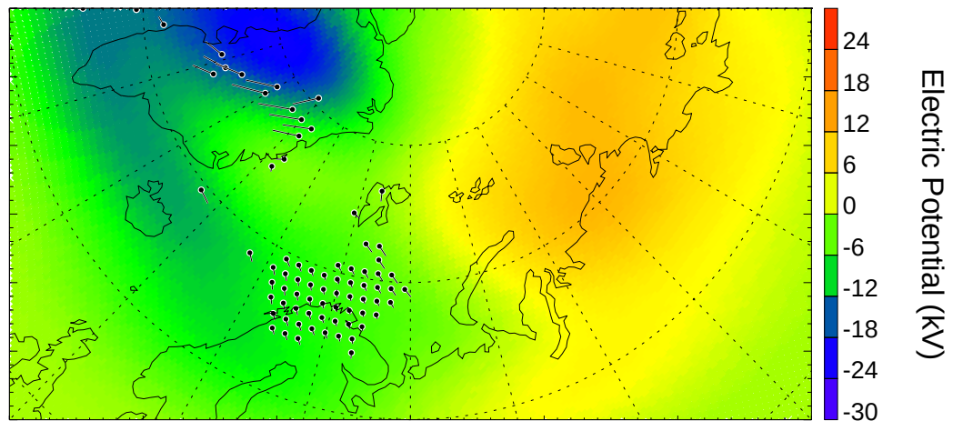
Electric Potential from SuperDARN 20:24:00 - 20:26:00 UT
