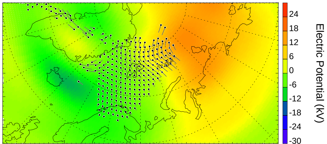
Electric Potential from SuperDARN 20:38:00 - 20:40:00 UT
