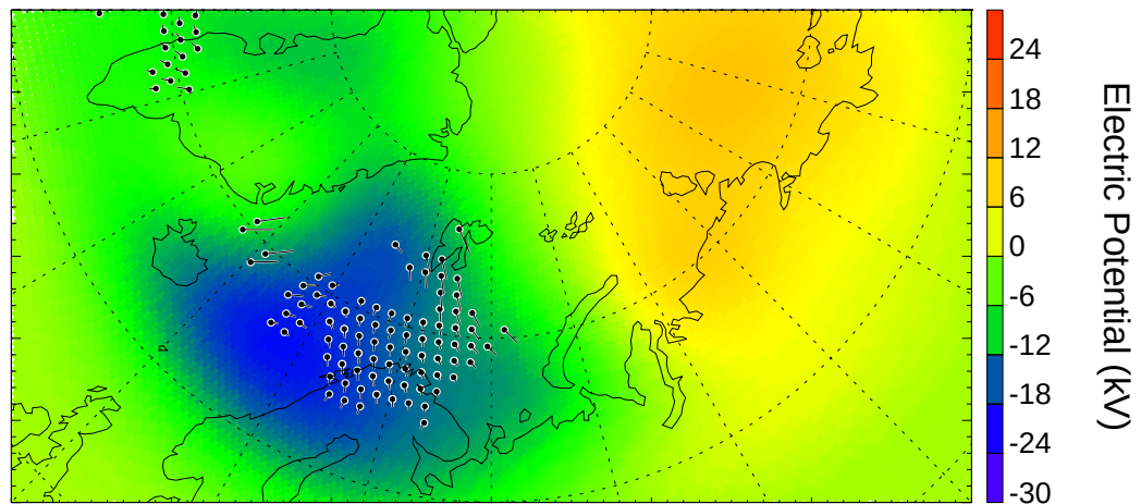
Electric Potential from SuperDARN 20:26:00 - 20:28:00 UT
