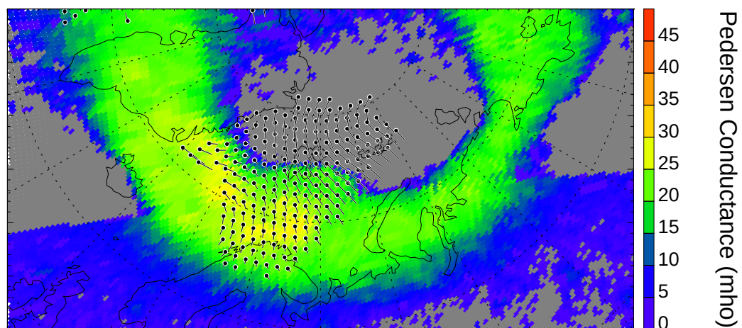
Pedersen Conductance from IMAGE/WIC
