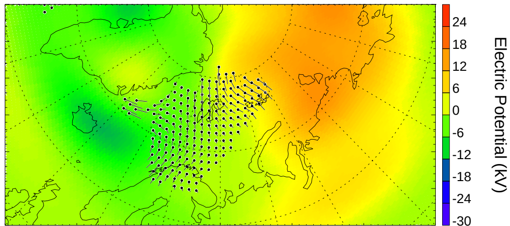
Electric Potential from SuperDARN 20:34:00 - 20:36:00 UT
