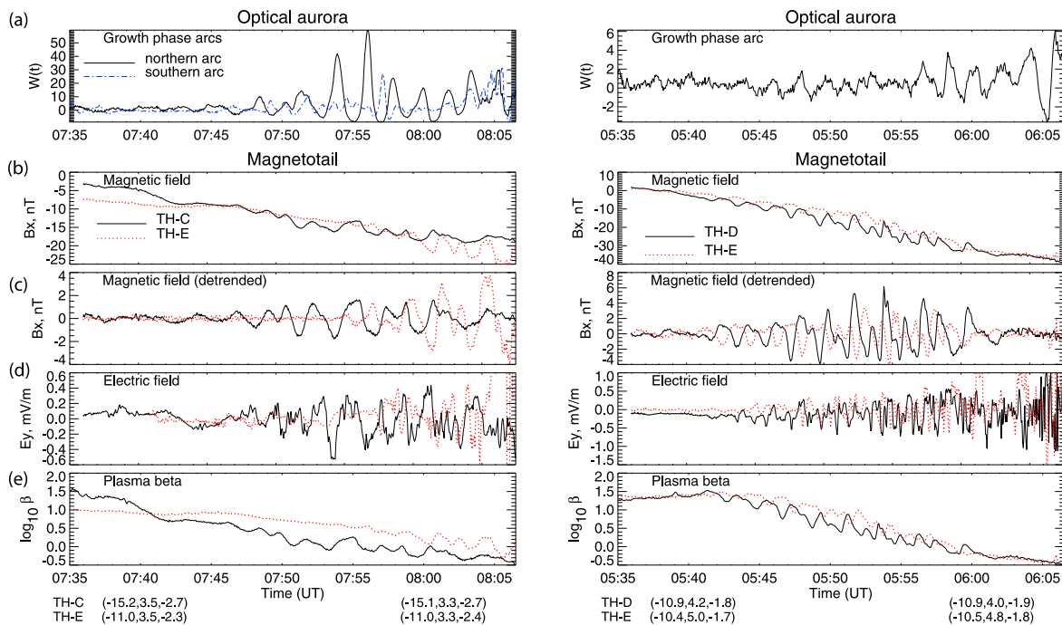
Figure 3. Simultaneous low-frequency wave oscillations (a) in the optical aurora and (b–e) in the CPS as measured by THEMIS probes, prior to the substorm onsets of (left) 03/03/08 and (right) 03/05/08. GSM coordinates of the probes are shown below the plots.
