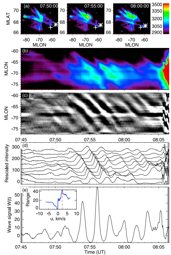
Figure 1. (a) Sample images of the pre-onset aurora observed by the Fort Simpson ASI on 03/03/08. Ionospheric footprints of TH-C and TH-E are shown with stars and crosses, correspondingly. (b) Raw ewogram a(\phi, t) representing time evolution of the northern arc seen in Figure 1a. (c) Detrended ewogram A(\phi, t) exhibiting westward-propagating periodic fronts of auroral intensity. (d) Stack plot of time-varying auroral intensity at different magnetic longitudes ( -70 to -60 MLon, bottom to top). (e) Wave signal W(t) extracted from A(\phi, t) using the surfing average technique. The inset shows the dynamical range of w(t, u) with a clear maximum at u = v_y = 2.3 km/s.
