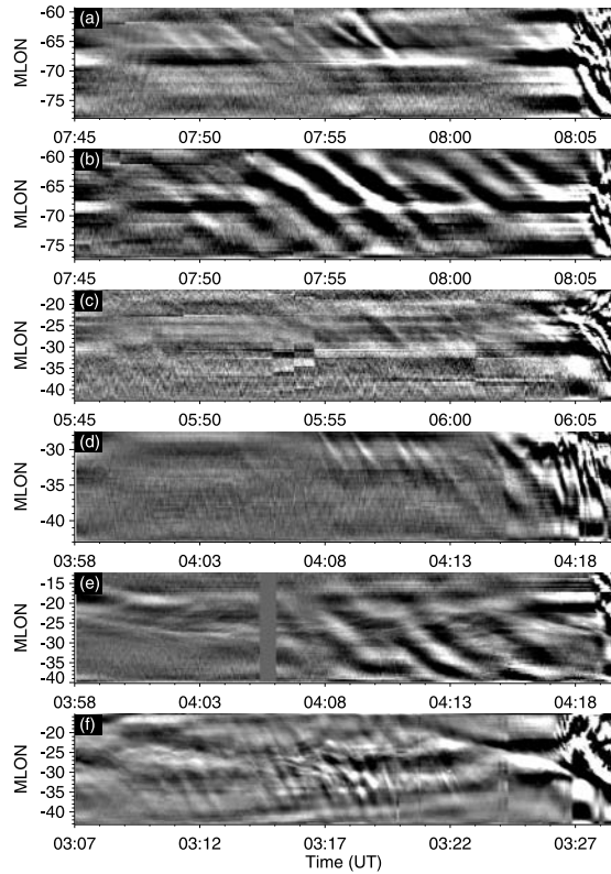
Figure 2. Detrended ewograms of six growth phase arcs showing westward traveling wave patterns: (a) 03/03/08, southern arc; (b) 03/03/08, northern arc; (c) 03/05/08; (d) 03/15/08, southern arc; (e) 03/15/08, northern arc; (f) 03/28/08.
